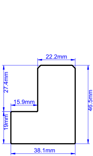
46.5mm Chamfer L Frame
