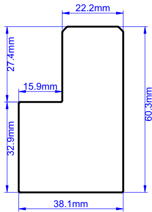
60.3mm Chamfer L Frame
