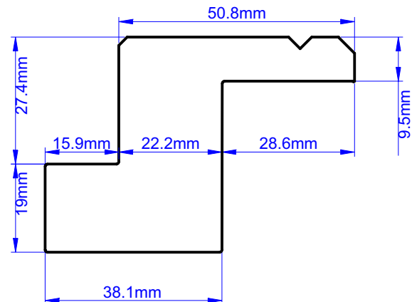
50.8mm Serrate Z frame
