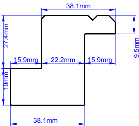
38.1mm Serrate Z frame
