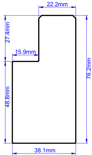
76.2mm Chamfer L Frame
